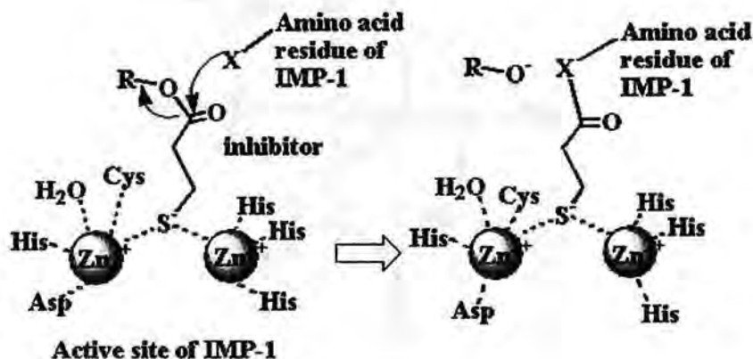
Figure 1. Irreversible inhibition mechanism.
