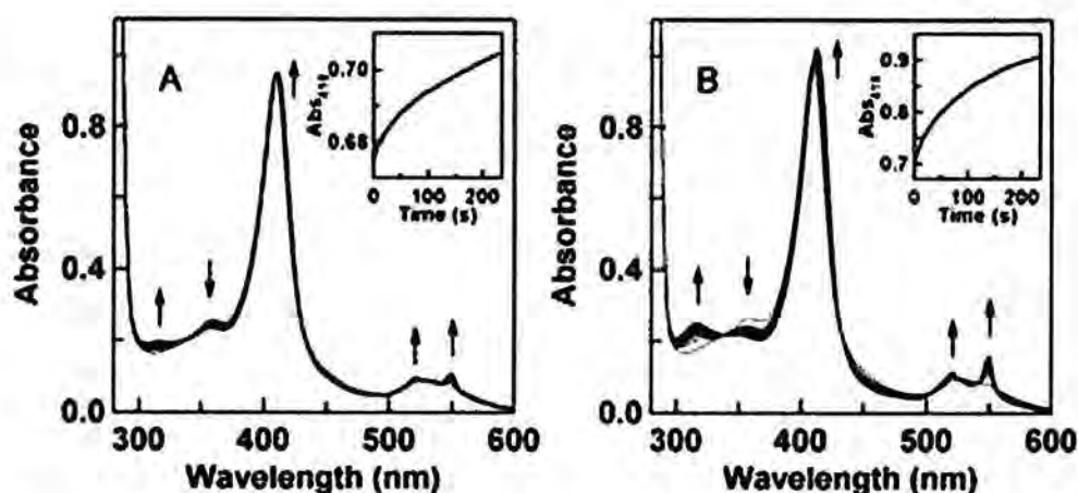
Figure 1. Absorption spectral changes of oxidized cyt c by reduction with TyrTyrPhe. Absorption spectra were taken each 30-min for 4 h. Inset: Time course of the absorption change at 418 nm.
