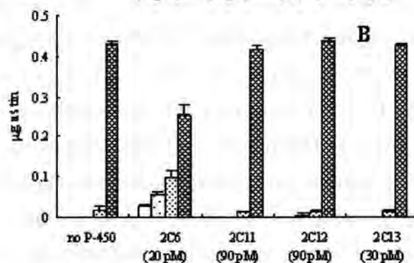
Fig. 2 In vitro metabolism of triphenyltin with cDNA-expressed rat CYPs of typical PB-inducible (A) and the 2C subfamily (B). No P-450 (vehicle control), containing baculovirus vector only. Values represent the mean \pm S.D. of four assays.
