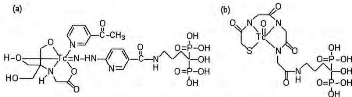
Figure 1. Structures of Tc-HYNIC-HBP (a) and Tc-MAG3-HBP (b).
