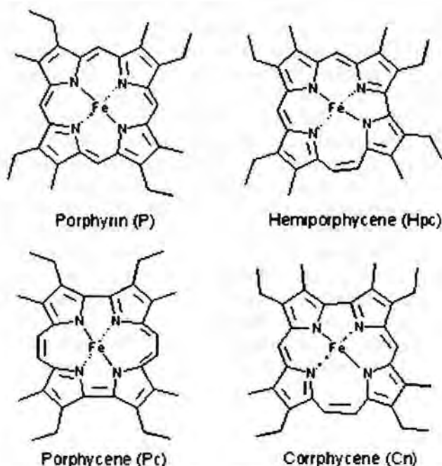
Figure 1 Structure of porphyrin and isomeric porphyrinoids
