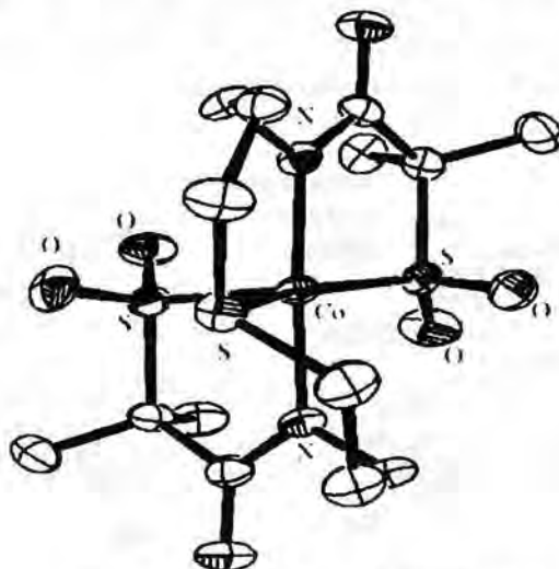
Figure Crystal structure of [Co(dpds-O 4 )] -
