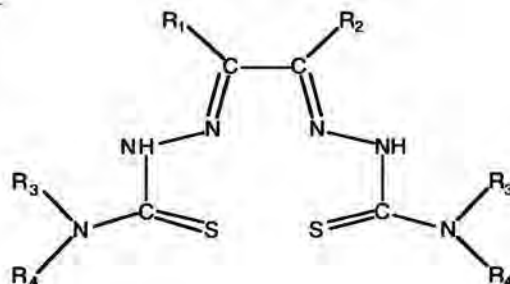
Structure of Dithiosemicarbazone Derivatives
