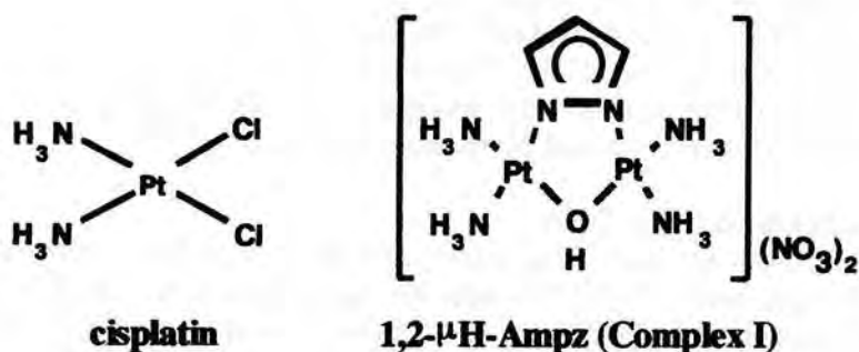
Structures of cisplatin and platinum(II) complexes
