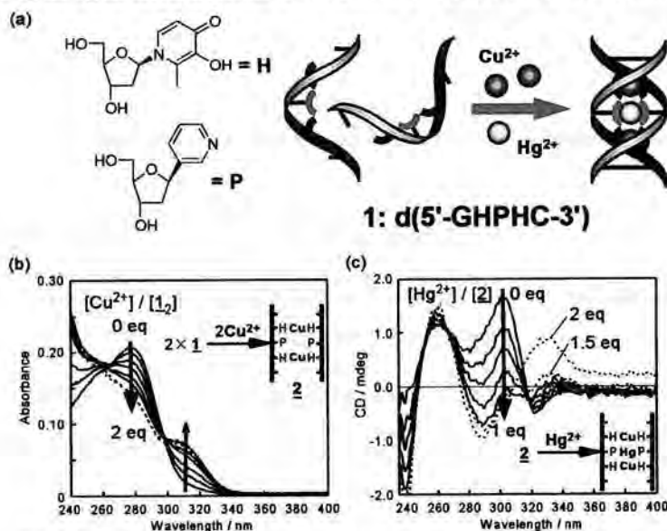
Fig. 1. (a) Schematic representation of hetero metal-assembly in artificial DNA. (b) UV absorption changes and (c) CD spectral changes of d(5'-GHPHC-3') at various concentrations of \text{Cu}^{2+} and \text{Hg}^{2+} ions at 25 °C. [Duplex] = 2.14 \mu\text{M} , 2 mM HEPES (pH 7.0), 5 mM \text{NaNO}_3 .
