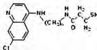
QuinolineC n SH
