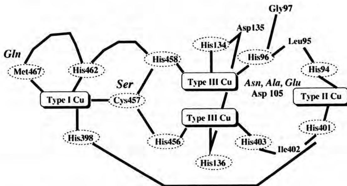
Fig. 1 Correlation of the Amino Acids around the Metal Binding Sites of BO
